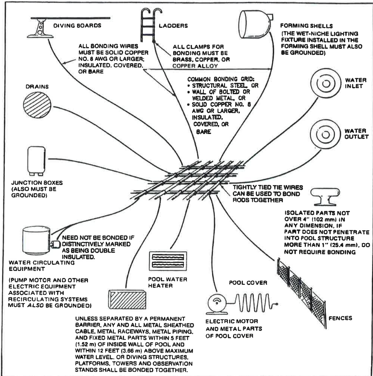
Fig. 30-4 Bonding the metal parts of swimming pool installations.
